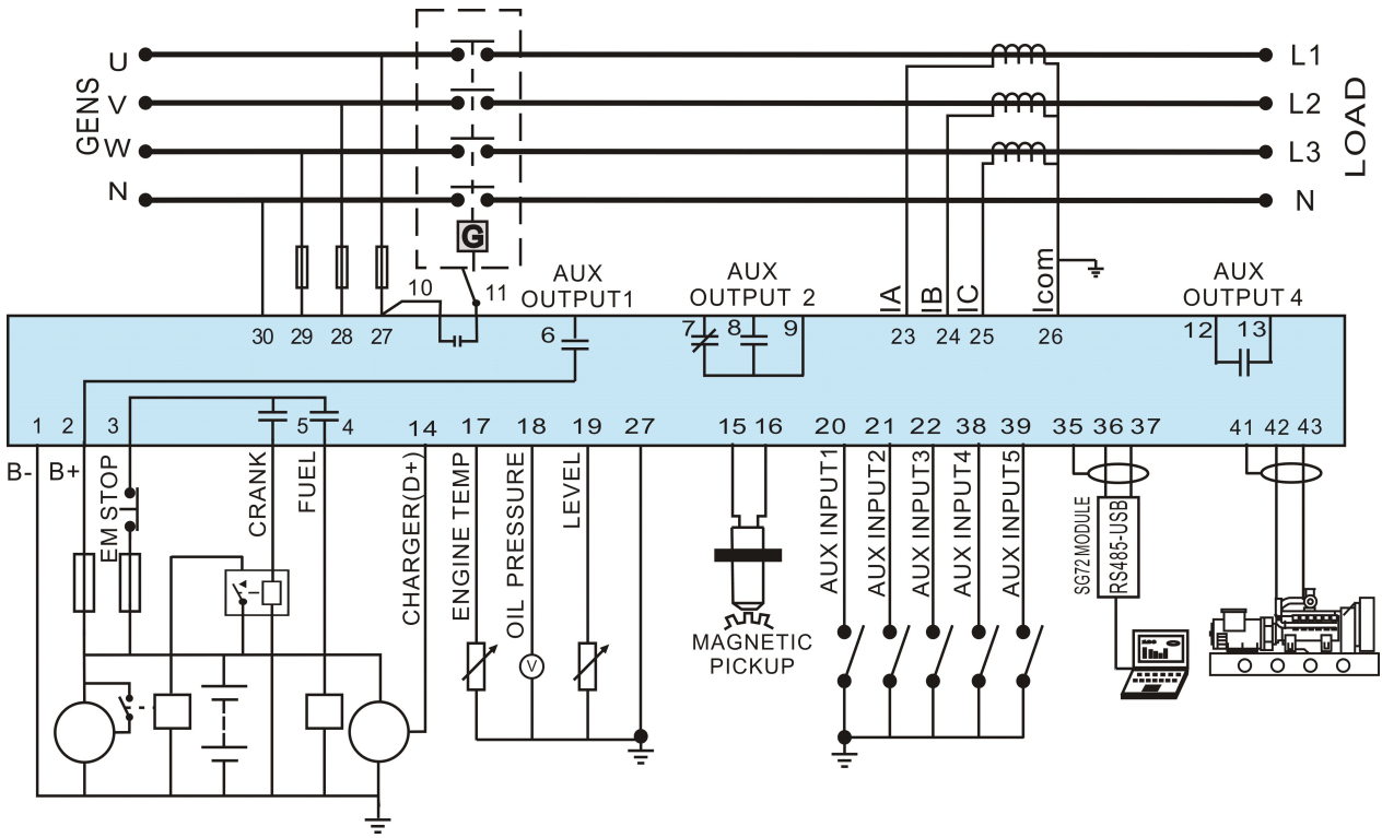
WHC6110CAN Typical Application Diagram
