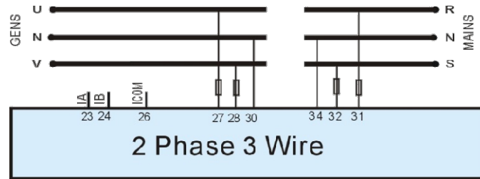
2 Phase 3 Wire
